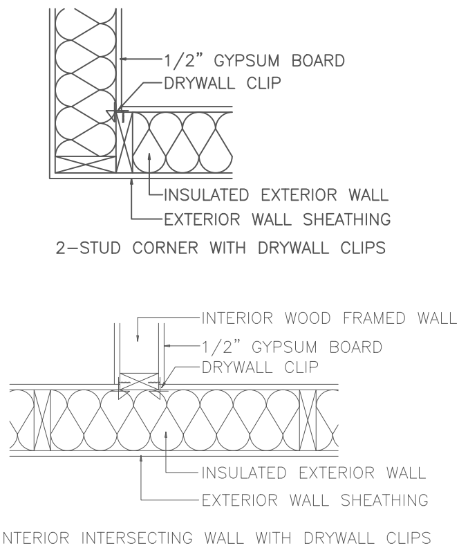
INTERIOR INTERSECTING WALL WITH DRYWALL CLIPS
